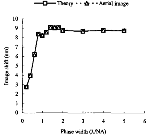
Fig. 2. Comparison between \Delta \hat{x}_c computed from Eq. (11) and that from aerial image simulation when \sigma = 0.5 .
