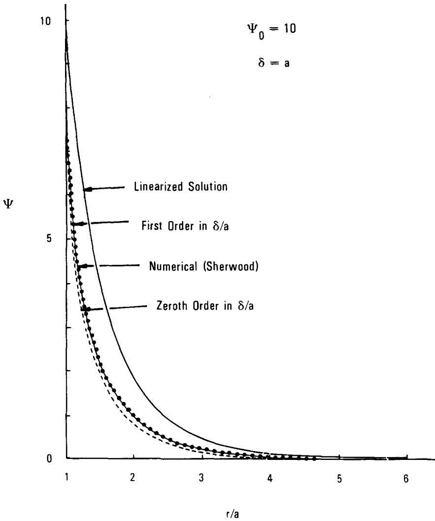
FIG. 1. Potential as a function of distance r/a ( a being the particle radius) for a high zeta potential \Psi_0=10 . The extreme case of \delta=a is shown here. The dashed line corresponds to the zeroth order term in Eq. (16), while the dotted line corresponds to the full Eq. (16).
