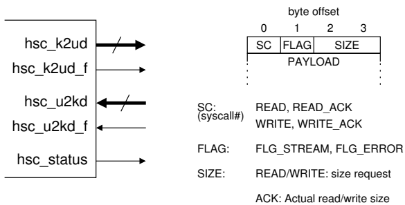
Fig. 3: Left: One copy of ioc with which BORPH’s hardware system call interface is built. Right: Format of packet transmitted through hsc.
