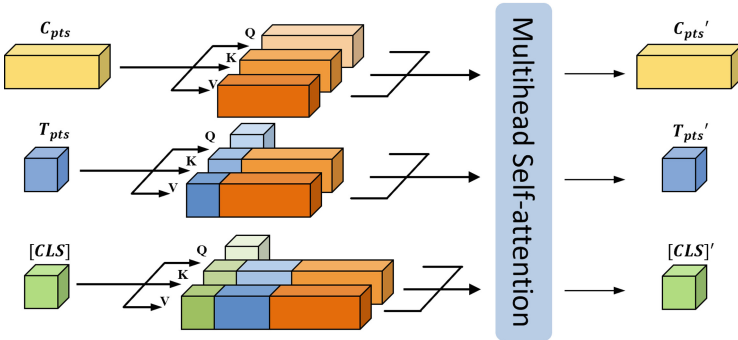
Fig. 3. Multimodal Self-attention. C-pts with known 3D coordinates attend to each other, while each of the T-pts attends to itself as well as the C-pts. [CLS] attends to all available C-pts and T-pts for object-level representation. For better visual effect, we show one T-pt doing self-attention in the middle row. Best viewed in color. (Color figure online)
