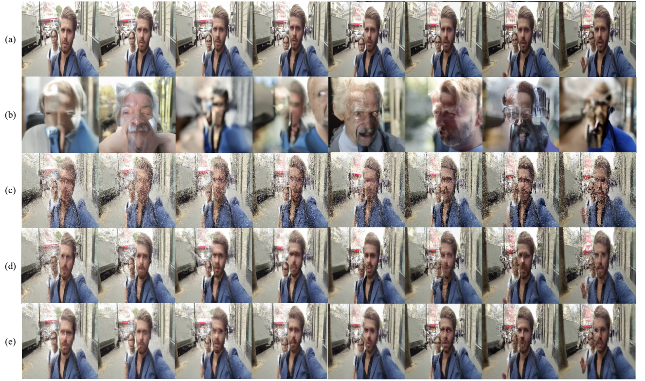
Fig. 3: (a) The original video frames in the video Human , and reconstruction results of the measurement using (b) conditional reverse-time SDE, (c) proximal optimization, (d) modified proximal optimization, (e) integration with pre-existing methods, respectively.
