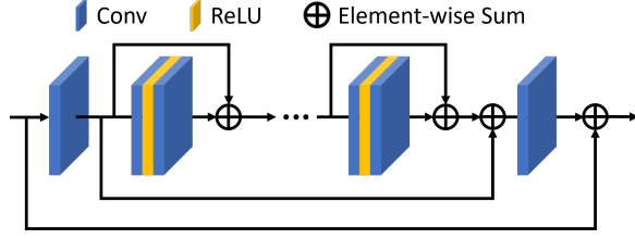
Fig. 2. Network architecture. This network consists of 1 convolutional layer, 16 residual blocks, and 1 convolutional layer. A long skip connection from head to tail is adopted to enable the residual learning.
