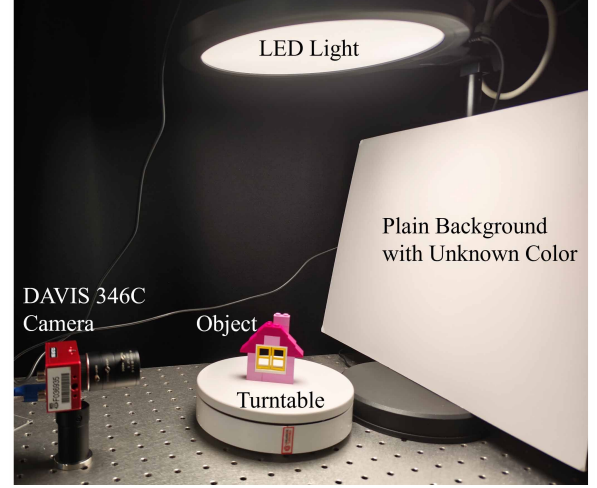
Fig. 2. Demonstration of Hardware Setup.
