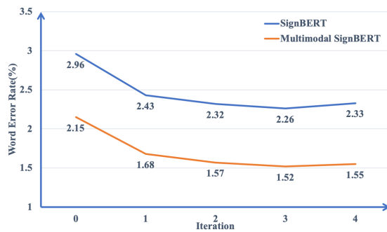
FIGURE 8. The experimental results of the iterative training.
