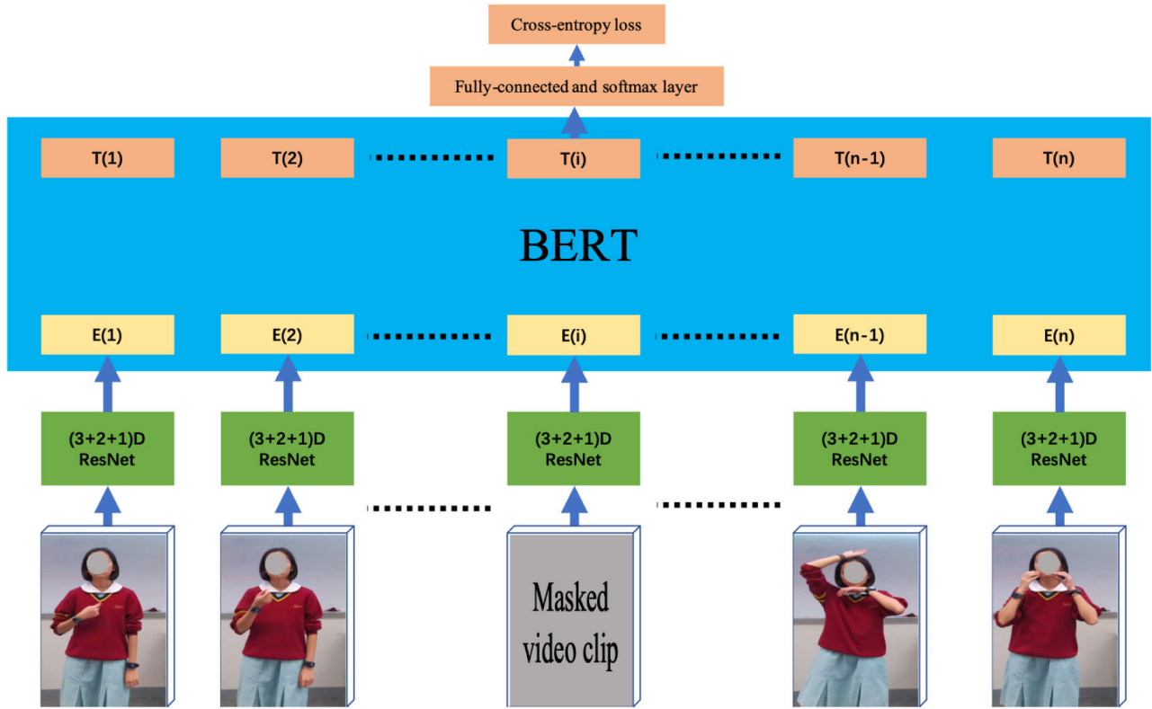
FIGURE 7. Training the BERT model with masked input.
