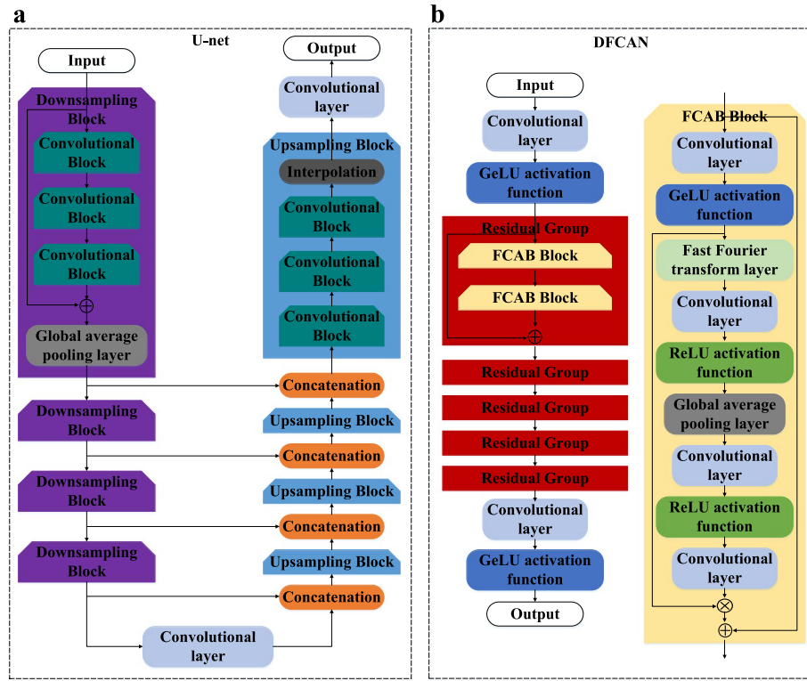
Fig. 2 The architecture of the generator of TCAN. (a) The architecture of U-net. (b) The architecture of DFCA
