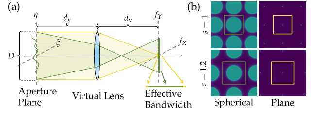
Fig. 2. (a) Fourier transform interpreted as a virtual thin lens model. The green and yellow areas denote spherical and plane waves, respectively. (b) Influence of oversampling factor. The inner squares indicate the sampling region of a spherical wave (left) and a plane wave (right) with oversampling factor s of one (top) and 1.2 (bottom), respectively. A larger region is visualized than the sampling rate to illustrate the aliasing artifact.
