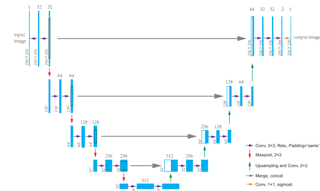
Fig. 2. The architecture of U-net. 'Conv, 3 \times 3 ' represents a 3 \times 3 convolution kernel with the ReLU activation function. 'Padding=same' means that the matrix dimensions of the input and output in the convolution layer are the same. 'Maxpool 2 \times 2 ' represents the function to choose the maximum value from a 2 \times 2 matrix. 'Upsampling and conv, 2 \times 2 ' stands for upsampling using a 2 \times 2 convolution kernel. Each blue box represents a multi-channel feature map, while the white ones represent the copied feature maps.
