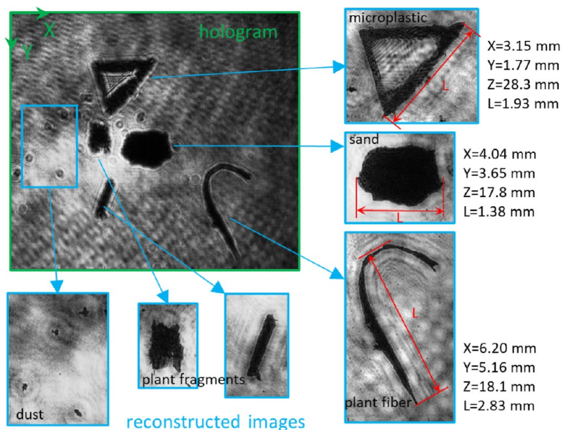
Figure 7. Numerical reconstruction of holograms for revealing particles' morphological features. The samples include an MP particle, sand, plant fiber and fragments, and dust, showing characteristic shapes, sizes, and 3D locations.
