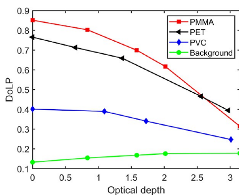
Figure 11. Evolution of DoLP of PMMA, PET, and PVC particles and the background as a function of the media's optical depth.
