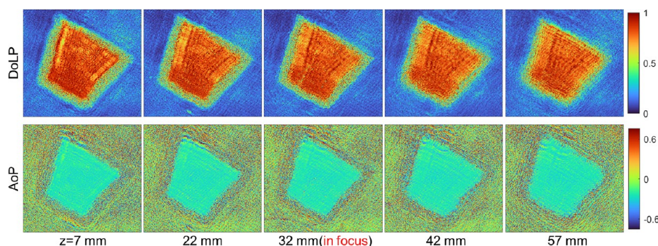
Figure 3. Evolution of DoLP and AoP of a PMMA particle as a function of the reconstruction distance. The images are reconstructed at one in-focus depth and four out-of-focus depths, respectively.
