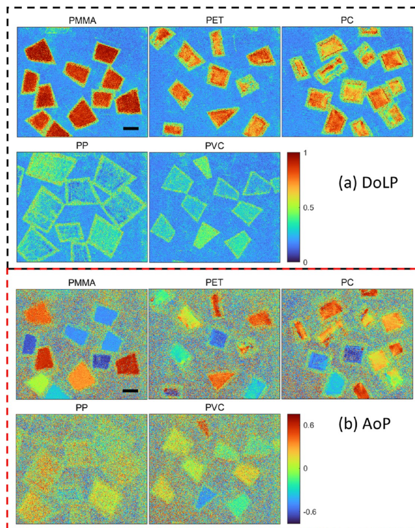
Figure 9. Color maps of DoLP and AoP for different MP samples. Scale bar: 1 mm.
