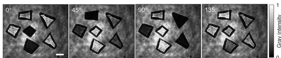
Figure 2. Representative holograms of MP particles in four polarization directions, which are captured in a single shot. Scale bar: 1 mm.
