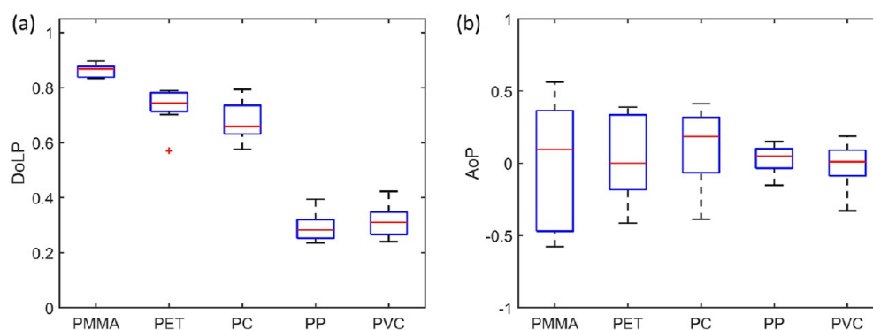
Figure 10. Visualization of the (a) DoLP and (b) AoP distributions of different MP samples using boxplots. The central red lines indicate the median, and the horizontal blue edges of the box are the 25th and 75th percentiles.
