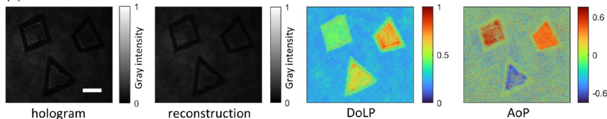
Figure 4. Image degradation due to scattering and absorption effects in the aqueous phase. The holographic and polarimetric images of MP particles in (a) pure water and (b) milk solution, respectively. Scale bar: 1 mm.
