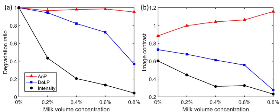
Figure 5. (a) Degradation ratio and (b) image contrast calculated based on the intensity, DoLP, or AoP, as a function of the volume concentration of milk solutions.
