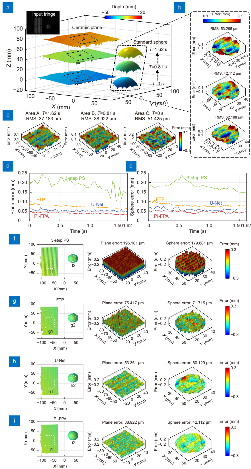
Fig. 5 | Precision analysis for a ceramic plane and a standard sphere moving along the Z axis. (a) 3D reconstruction results using PI-FPA at different time points. (b–c) the error distributions of the sphere and plane. (d–e) temporal precision analysis results of the plane and sphere over a 1.62 s period using 3-step PS, FTP, U-Net, and PI-FPA. (f–i) the color-coded 3D reconstruction and the corresponding error distributions of the plane and the standard sphere using different methods at T = 0.81 s.
