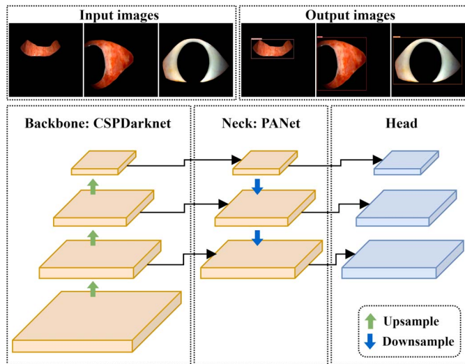
Fig. 2. YOLOv5 architecture for RGB image classification, featuring a CSPDarknet backbone for feature extraction, a PANet neck for feature fusion, and a head to output class (Normal, SCH, or bulbar conjunctivitis), score, and location.
