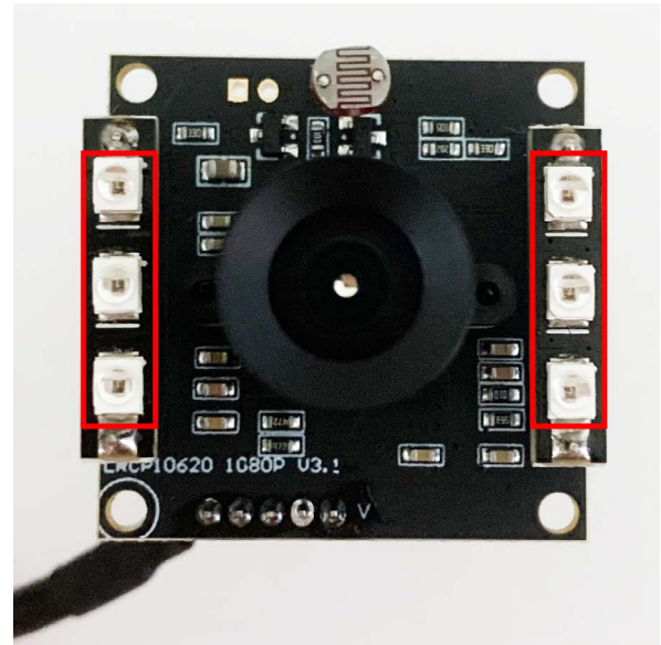
Fig. 16. A USB-enabled imaging sensor featuring an integrated IR LED array of 850 nm (highlighted in red box) designed for a portable meibography device.
