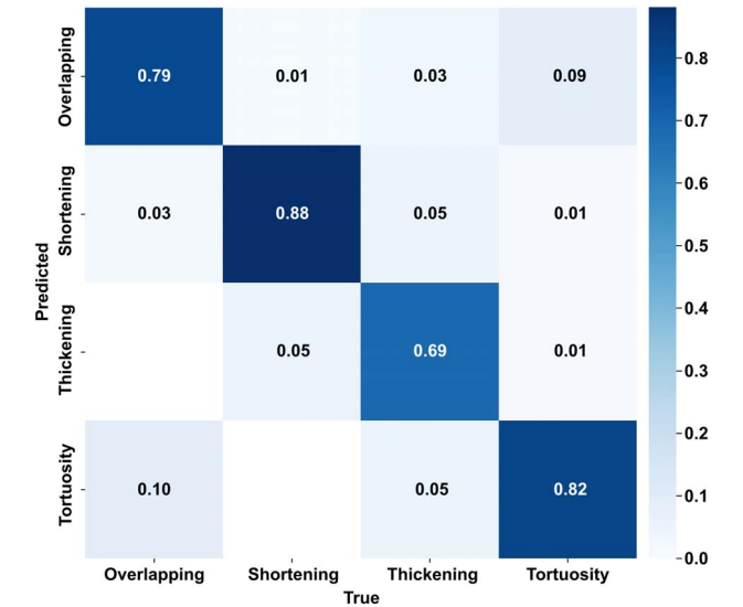
Fig. 12. The performance of the MG irregularity classification is quantitatively assessed using the confusion matrix. Four kinds of MG irregularities are overlapping, shortening, thickening, and tortuosity.
